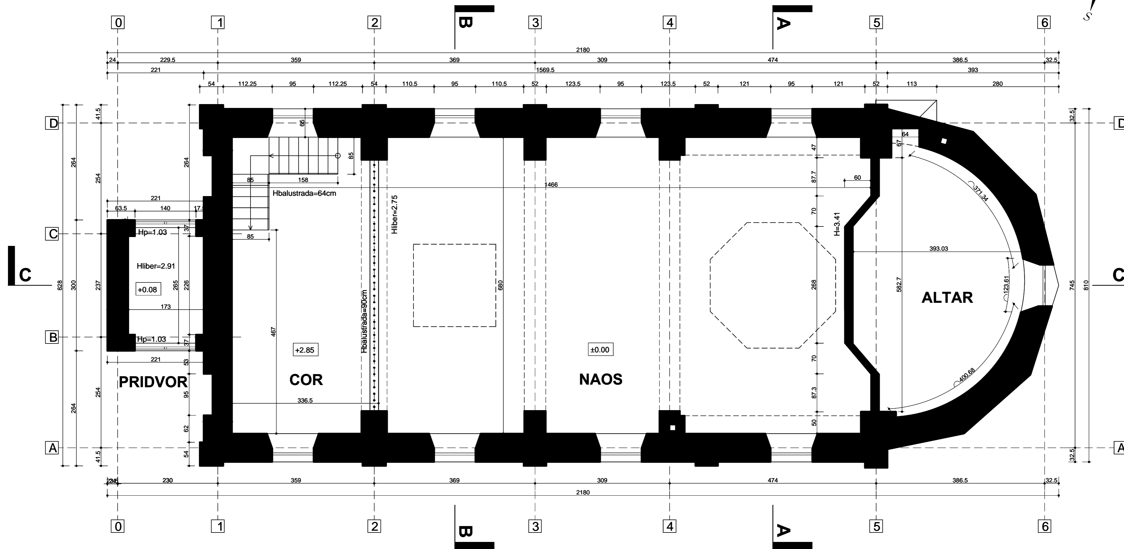
RELEVU COTA +2.85
